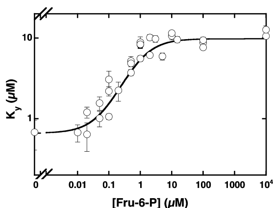
Figure 5. Plot of apparent dissociation constants ( K_y ) for PEP as a function of Fru-6-P concentration. The data were fit to eq 3b to obtain the dissociation constants for Fru-6-P ( K_{ia}^0 ) and the coupling constant Q_{ay} .
