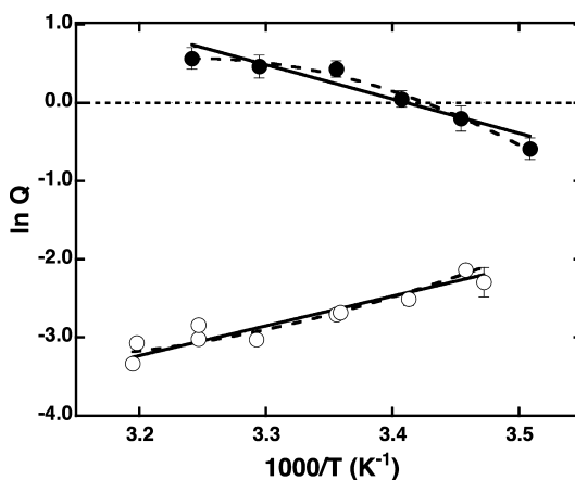
Figure 3. van't Hoff plots of \ln Q_{ay} (open circle) and \ln Q_{ax} (closed circles) as a function of temperature. The data were fit to eq 6b (solid line) to obtain the enthalpy component of coupling free energy or to eq 6a (dashed line) to obtain the enthalpy and change in the heat capacity at 25 °C.
