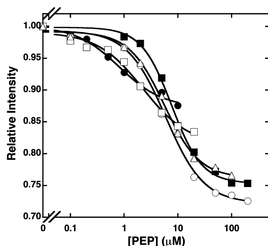
Figure 4. Plot of relative fluorescence intensity of the L313W variant at 25 °C as a function of PEP concentration at Fru-6-P concentrations of 0 (solid circles), 0.2 (open squares), 1 (open triangles), 5 (open circles), and 100 \mu\text{M} (solid squares). The sample was excited at 295 nm, and the fluorescence intensity was detected using the 2 mm, 335 nm Schott cut-on filter.
