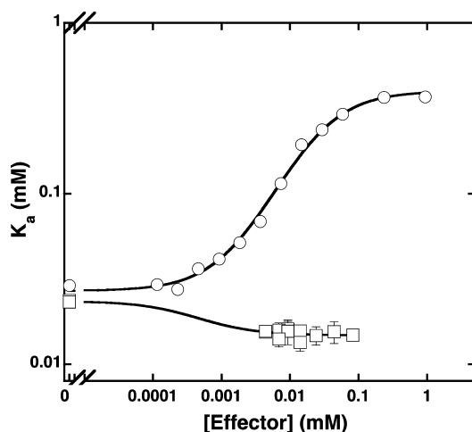
Figure 2. Plot of apparent dissociation constants ( K_a ) for Fru-6-P as a function of PEP (circles) or MgADP (squares) concentration at pH 8 and 25 °C. The data were fit to eq 3a to obtain the dissociation constants for PEP ( K_{iy}^o ) and MgADP ( K_{ix}^o ) as well as the coupling constants ( Q_{ay} and Q_{ax} ) reported in Tables 1 and 2.
